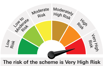
Scheme Risk-o-meter
